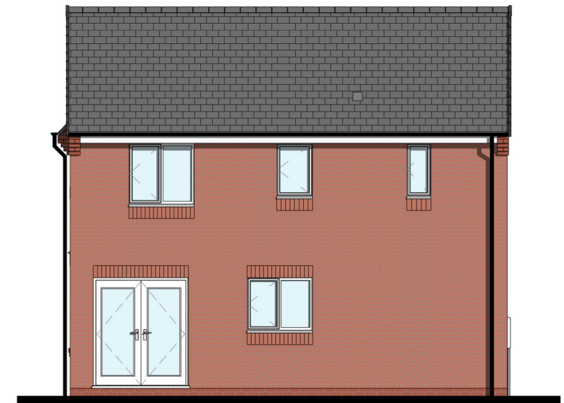
Rear Elevation
